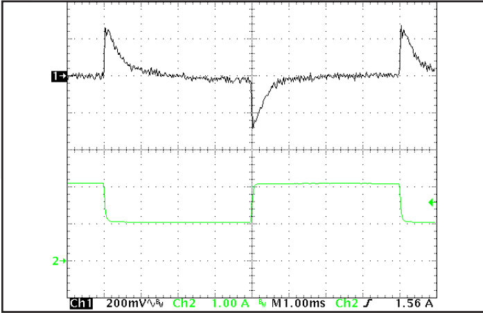
Figure 11: Output voltage response to step-change in load current 50%-100%-50% of Iout (max); dI/dt = 0.01 A/µs. No external load capacitance. Ch 1: Vout (200 mV/div). Ch 2: Iout (1 A/div). (1 ms/div).
